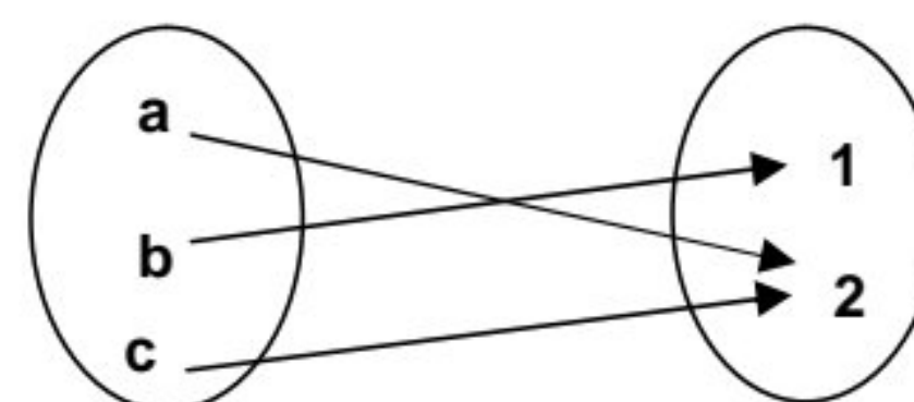
Surjective function
