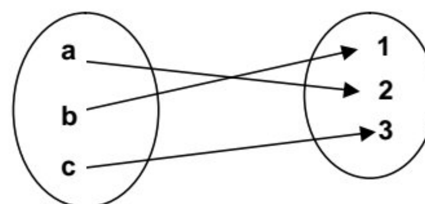
Bijective function
