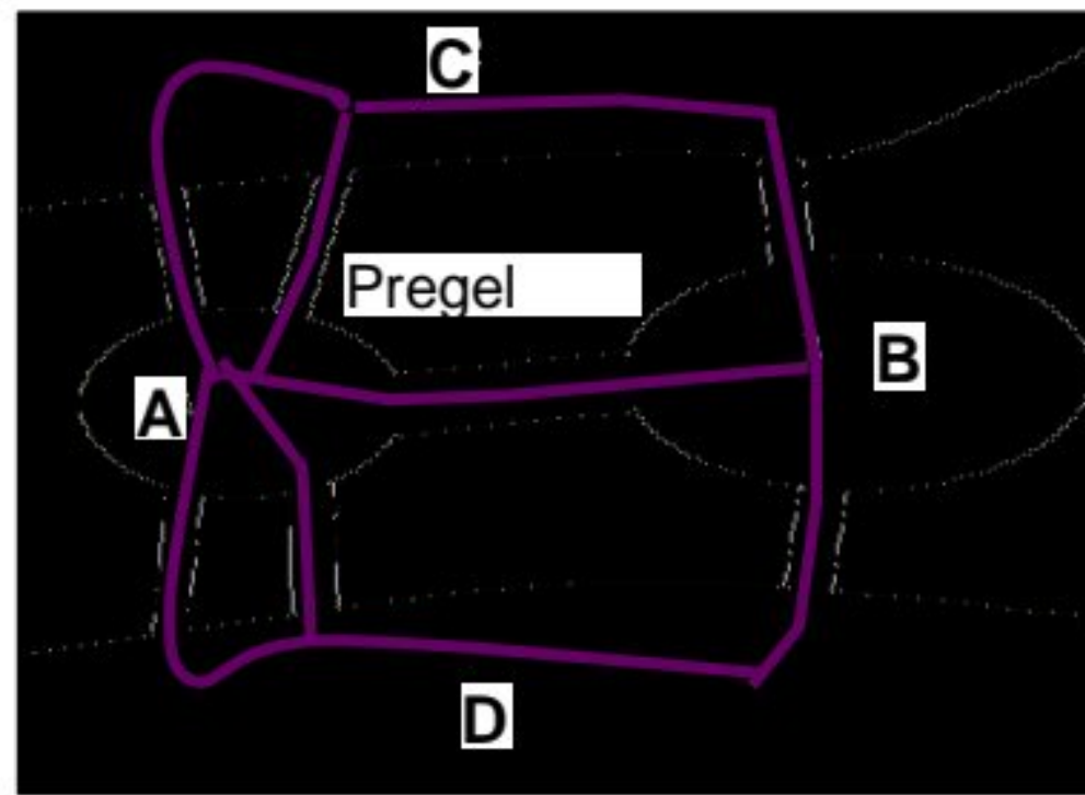
Figure 2: Representation of Seven bridges problem
