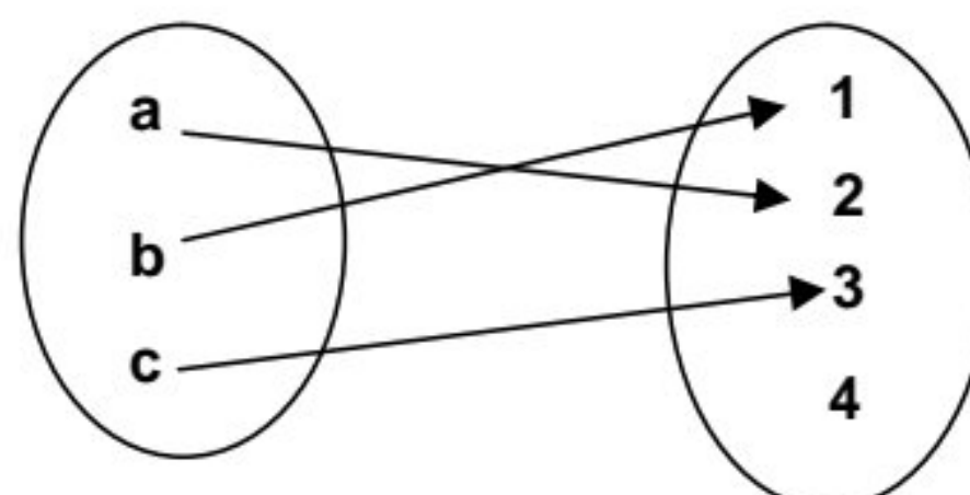
Injective function
