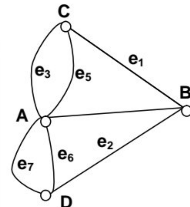
Figure 2: Representation of Seven bridges problem
