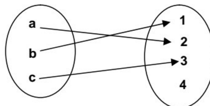
Injective function
