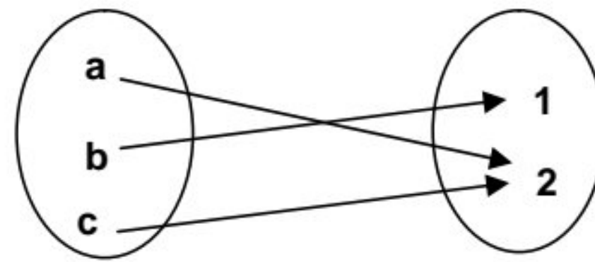
Surjective function
