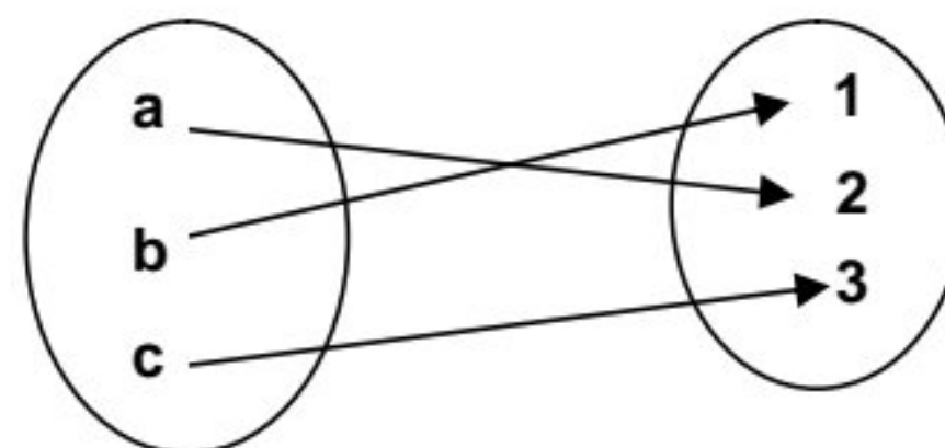
Bijective function
